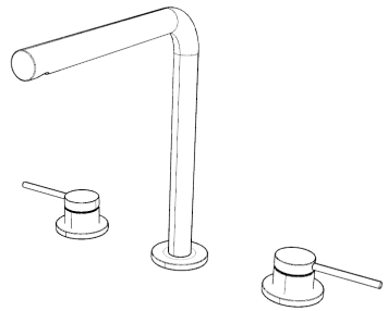
AB005106
