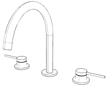
AB005006
