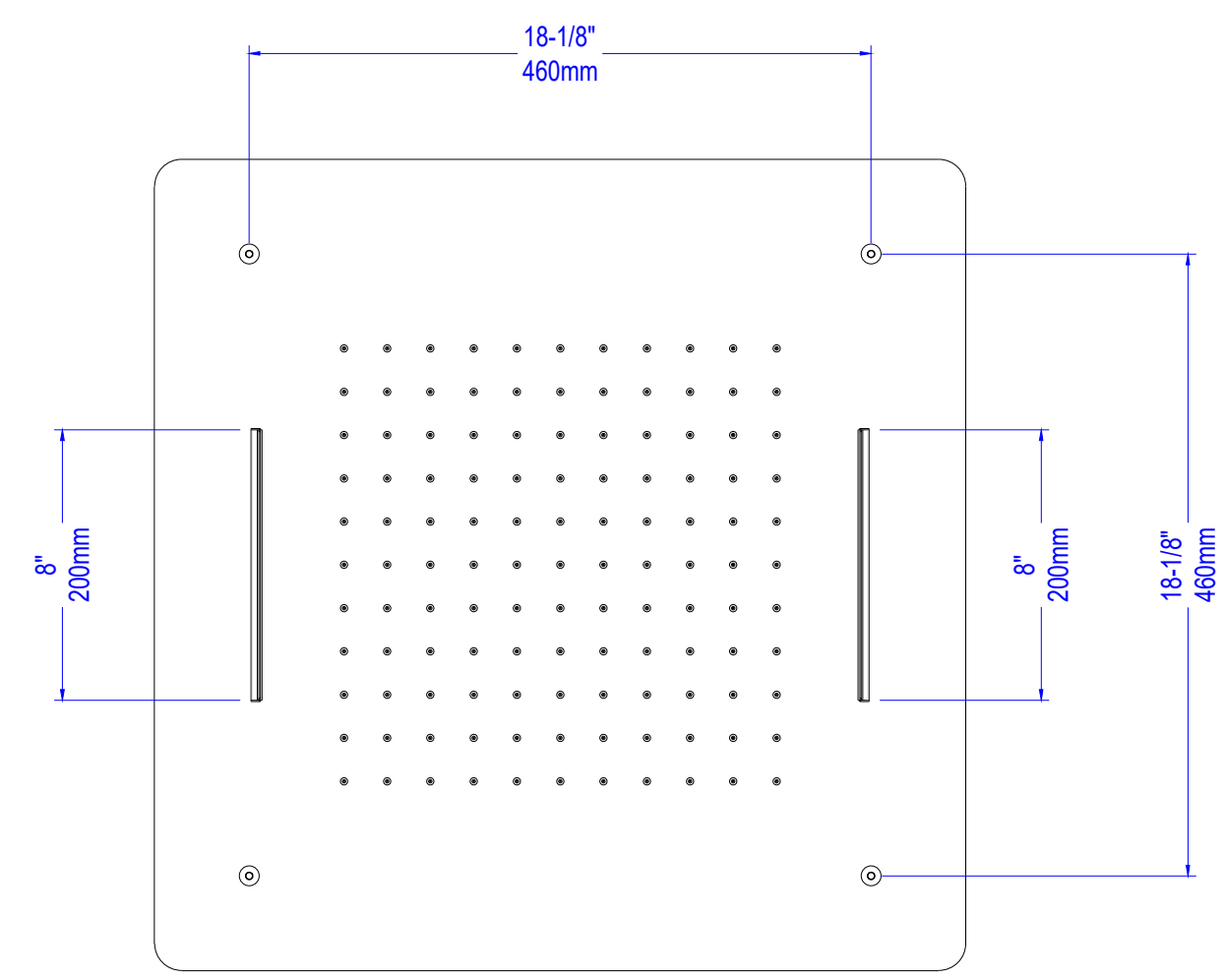
Silicone nozzles 121 PCS
